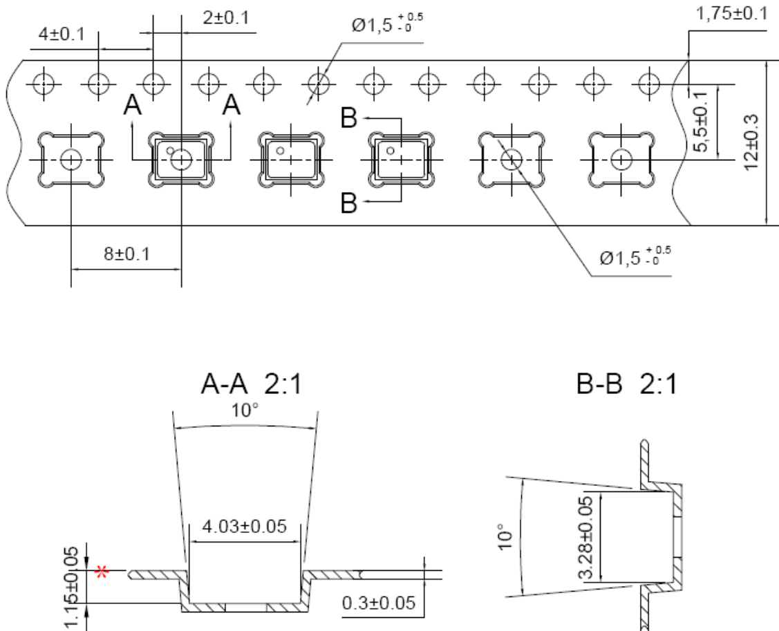
Figure 7: Carrier Tape (1)
