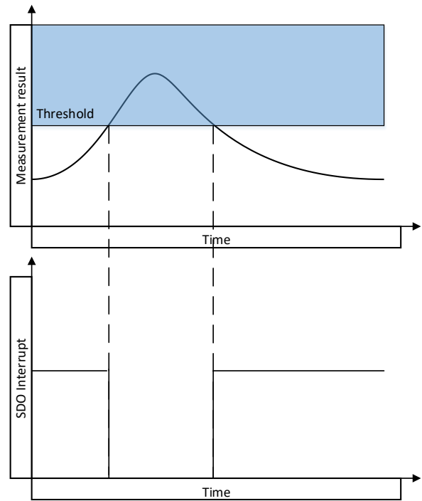
Interrupt mode 2: data>threshold (0x0D=0x04)
