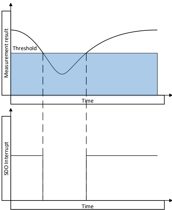
Interrupt mode 1: data<threshold (0x0D=0x02)
