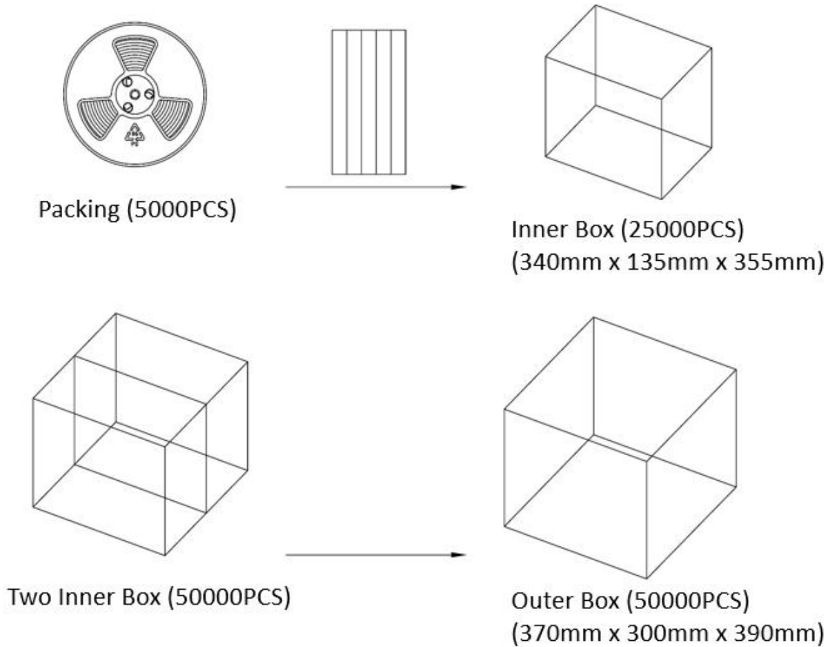
Figure 9: Packing Box
