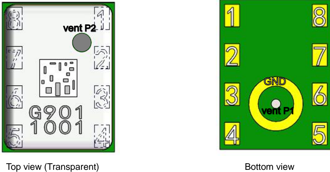
Figure 5: Layout pin configuration SPL03-001 (bottom view and top view)
