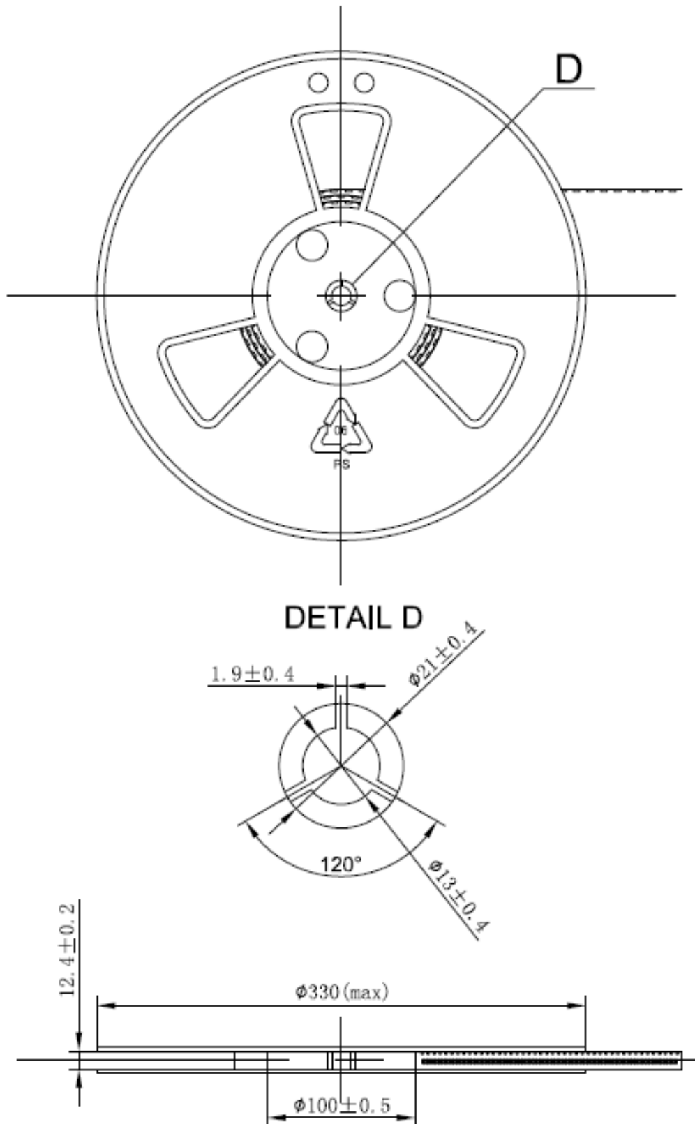
Figure 8: Carrier Tape (2)
