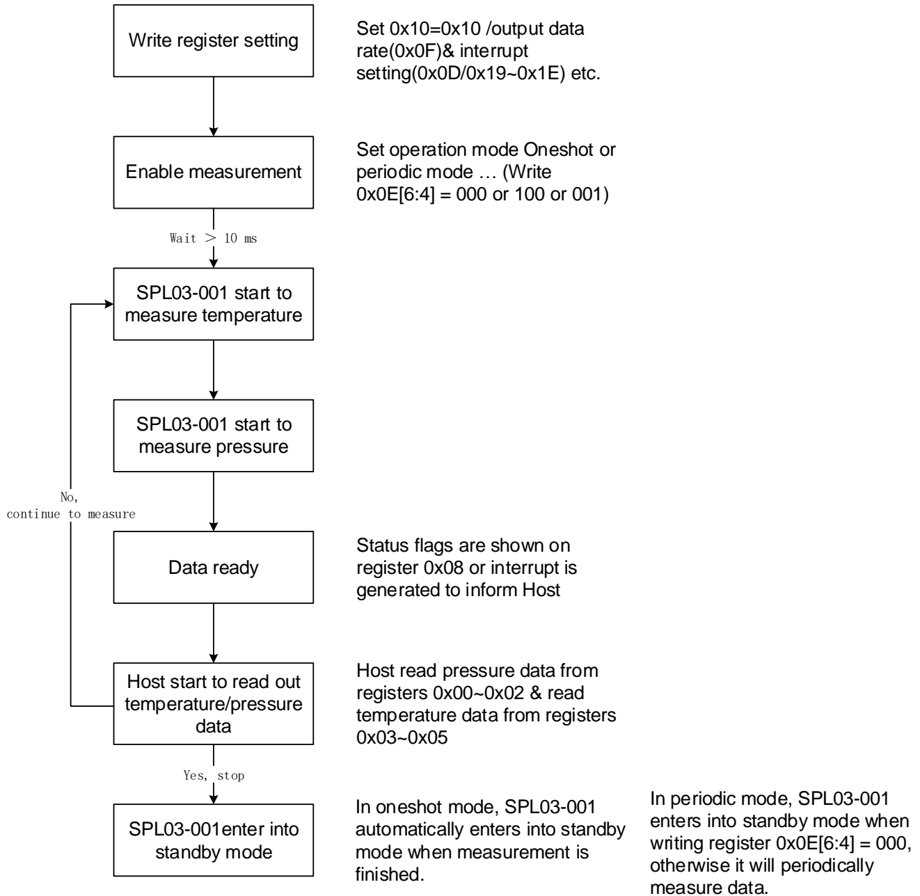
Figure 3: Measurement flow
