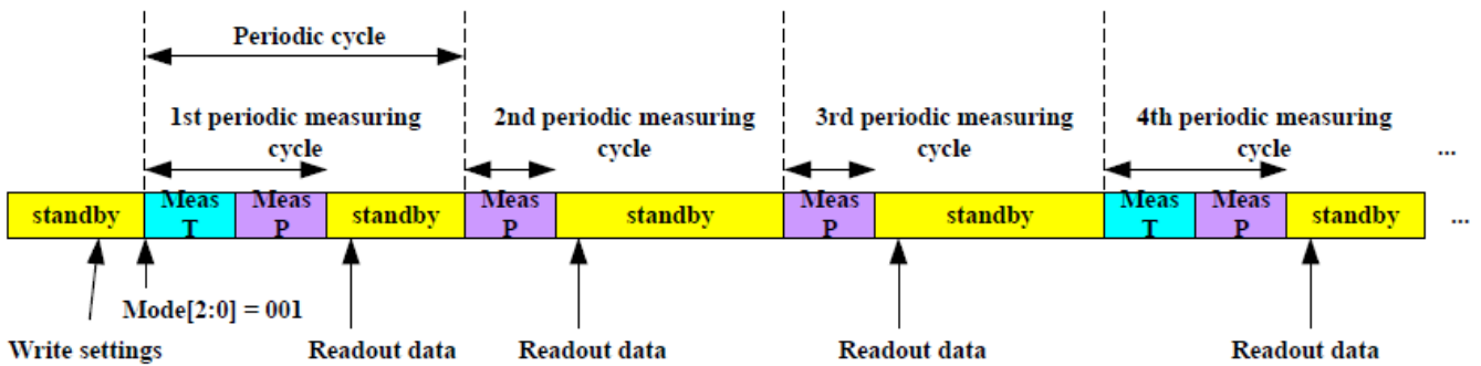
Figure 2: Periodic mode
