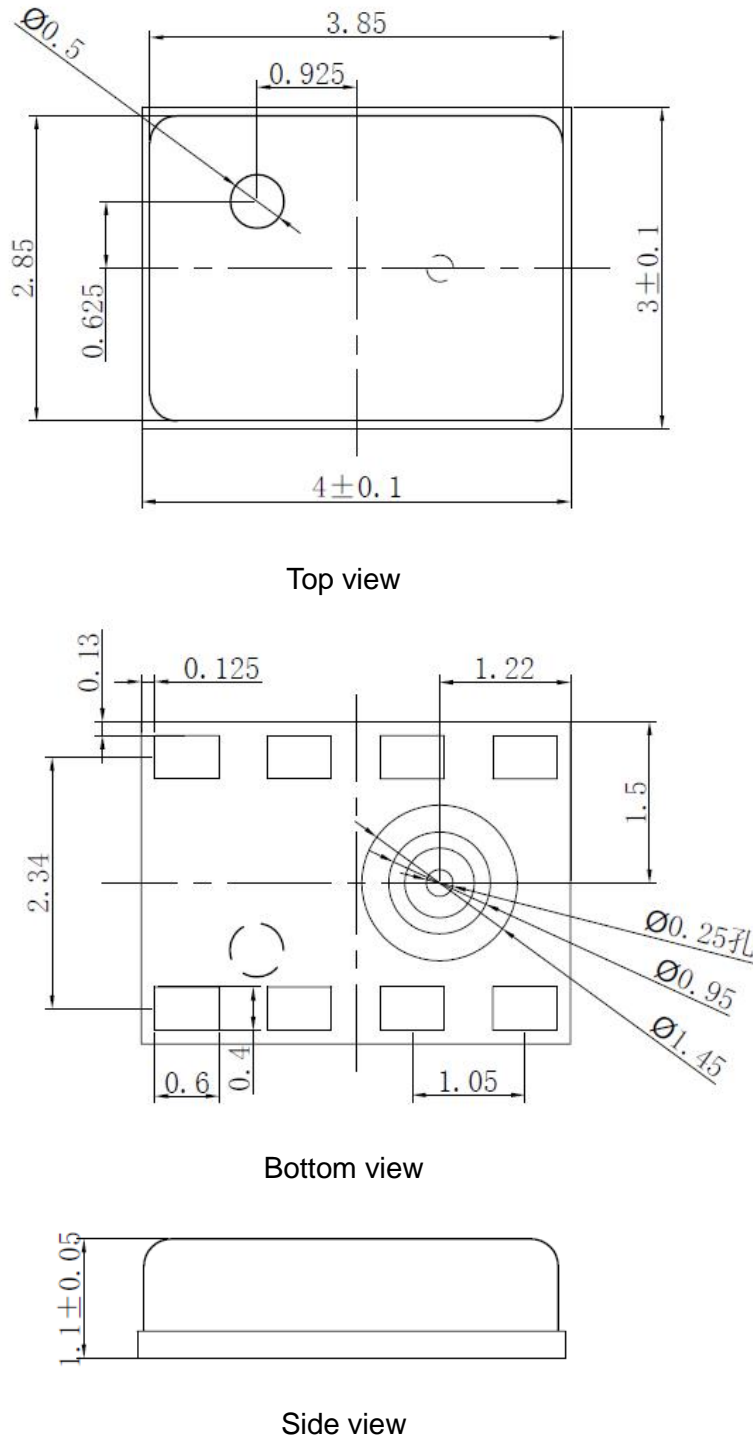
Figure 6: SPL03-001 outline and mechanical data
