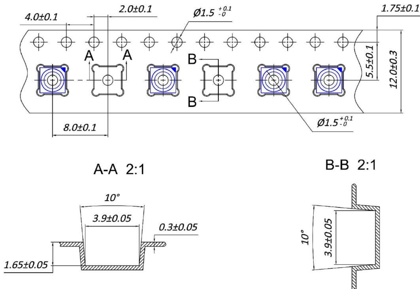
Figure 5: Carrier Tape (1)
