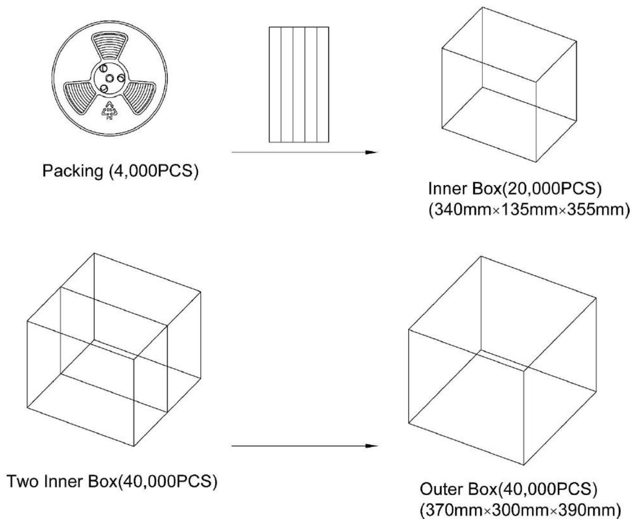
Figure 7: Packing Box
