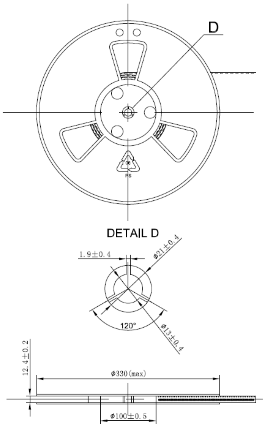
Figure 6: Carrier Tape (2)
