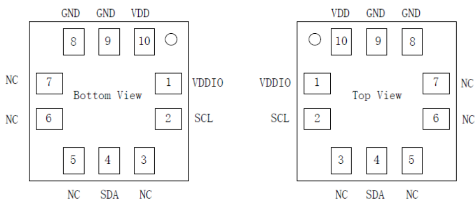
Figure 3: Layout pin configuration SPL16-001 (bottom and top view)
