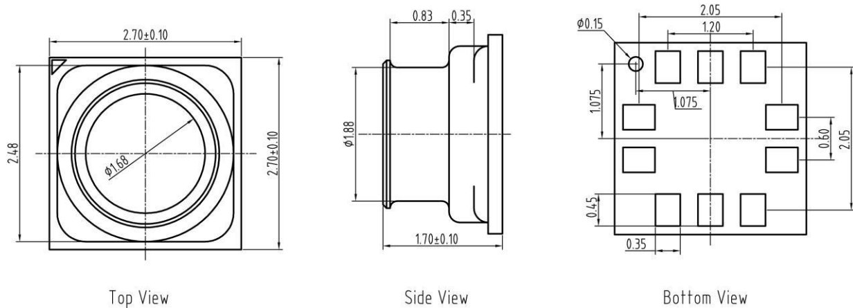
Figure 4: SPL16-001 outline and mechanical data
