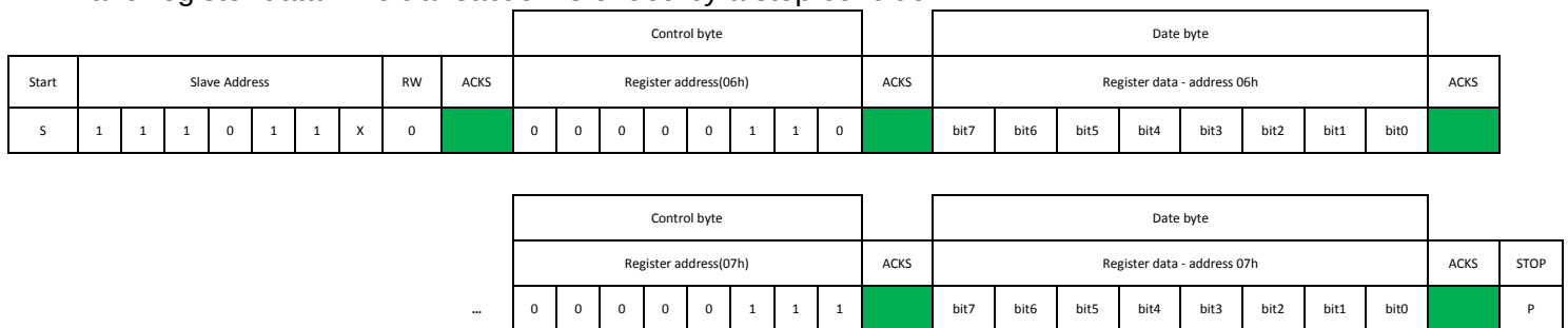
Figure 1: I2C write command
