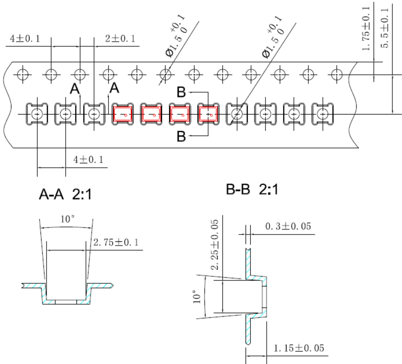
Figure 18: Carrier Tape (1)
