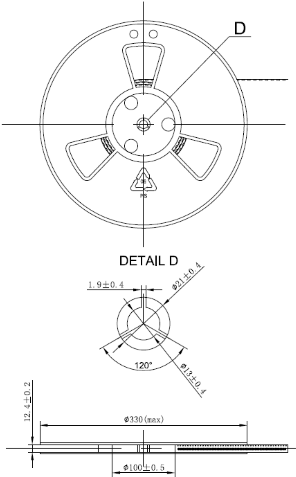
Figure 19: Carrier Tape (2)
